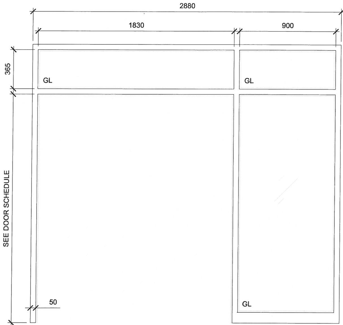
FRAME TYPE 7 DOUBLE DOOR W/ SIDE LIGHT / TRANSOM (LIBRARY)
