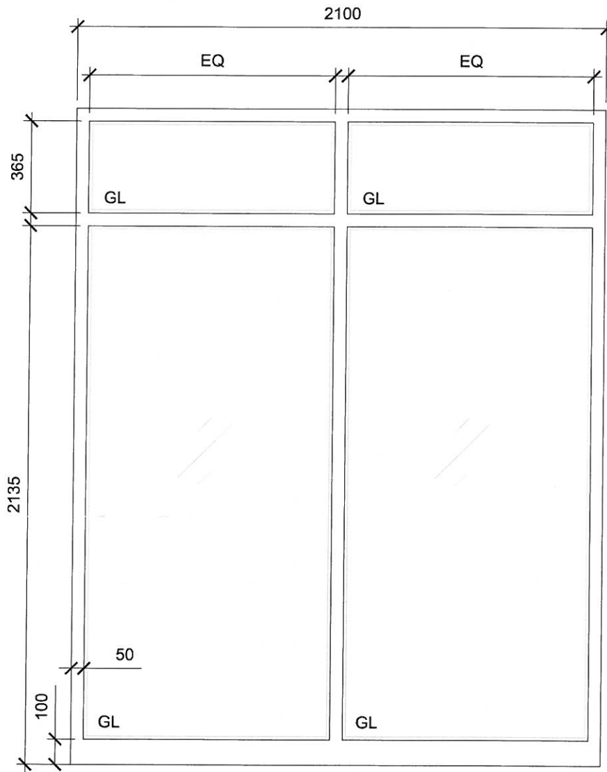
FRAME TYPE BL-3 GLAZING (LIBRARY)
