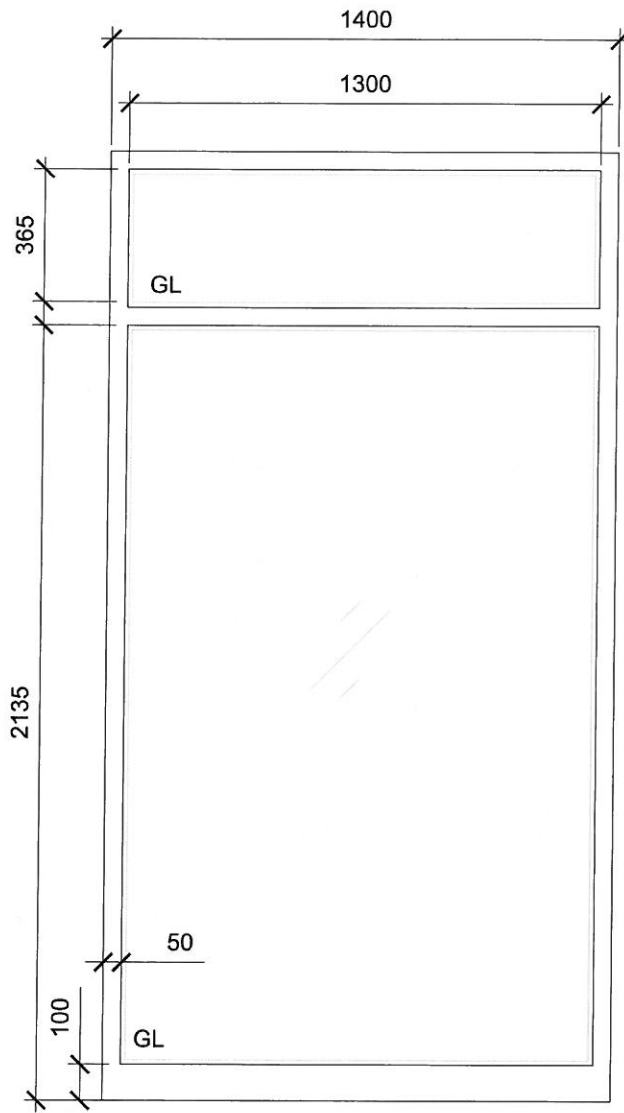
FRAME TYPE BL-4 GLAZING (LIBRARY)
