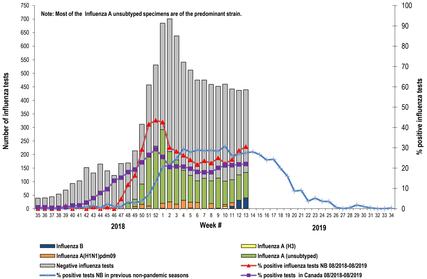
Graph 1: Number and percent of positive influenza specimens 2 in New Brunswick by week, up to March 30, 2019 (data source: G. Dumont Lab results)
