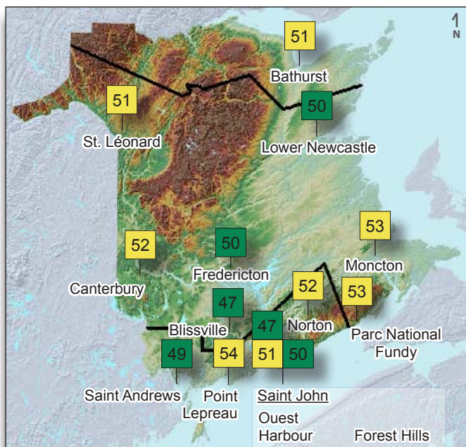
Ozone (ppb)
