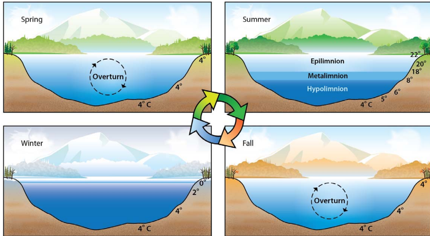
Figure 1. Lake seasonal thermal stratification and mixing
